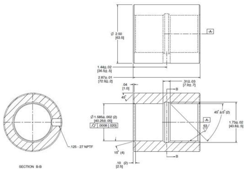
SECTION B-B
